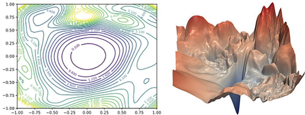
Figure 10.1 In this typical loss space, remember, this is the type of loss value we can feasibly get with our deep learning algorithms. On the left, you have 2D contour lines of equal loss, and on the right, you have a 3D rendering of what a loss space may look like. Remember the mountaineering analogy from chapter 6? (Source: “Visualizing the Loss Landscape of Neural Nets,” by Tom Goldstein et al., 2018, https://github.com/tomgoldstein/loss-landscape .)
