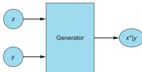
Figure 8.1 CGAN Generator: G(z, y) = x^*|y . Using random noise vector z and label y as inputs, the Generator produces a fake example x^*|y that strives to be a realistic-looking match for the label.
