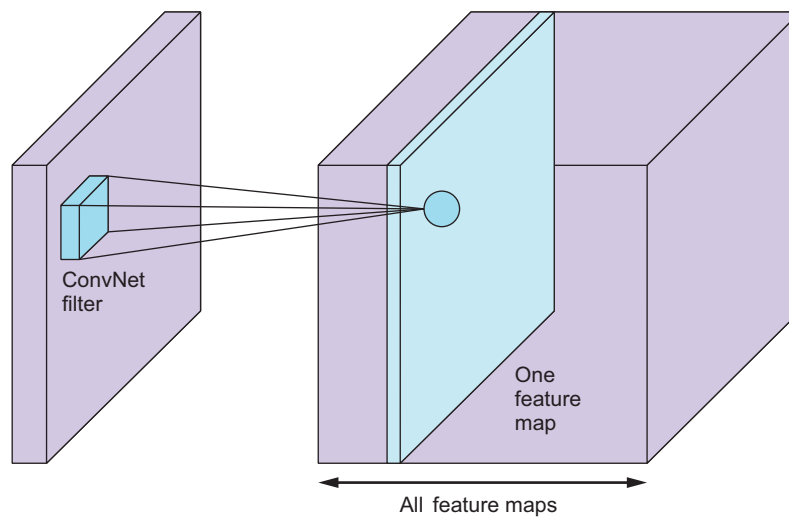
Figure 4.2 An activation value for a single convolutional step within the context of the activation map (feature map) and the input and output volumes. Notice that the ConvNet filter extends through the full depth of the input volume and that the depth of the output volume is determined by stacking together activation maps.
