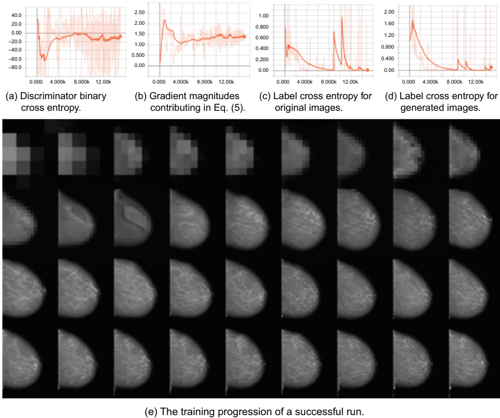
Figure 6.7 Progressive growing of FFDM. This is a great figure because it not only shows the progressively increasing resolution on these mammograms (e), but also some training statistics (a)–(d) to show you that training these GANs is messy for everyone, not just you.
