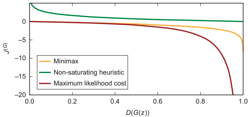
Figure 5.5 A sketch of what the hypothesized relationships are meant to look like in theory. The y-axis is the loss function for the Generator, whereas D(G(z)) is the Discriminator's “guess” for the likelihood of the generated sample. You can see that Minimax (MM) stays flat for too long, thereby giving the Generator too little information—the gradients vanish.
