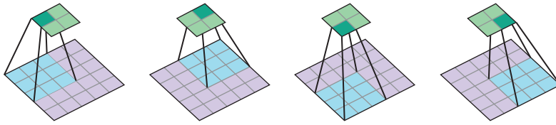
Figure 4.1 A 3 \times 3 convolutional filter as it slides over a 5 \times 5 input—left to right, top to bottom. At each step, the filter moves by two strides; accordingly, it makes a total of four steps, resulting in a 2 \times 2 activation map. Notice how at each step, the entire filter produces a single activation value.
