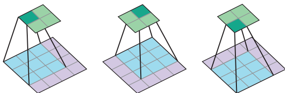
Figure 12.2 The output pixel ( 2 \times 2 patch) ignores anything except the small highlighted region. Attention helps us solve that.
