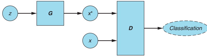
Figure 3.4 The Generator network G transforms the random vector z into a fake example x^* : G(z) = x^* . The Discriminator network D outputs a classification of whether the input example is real. For the real examples x , the Discriminator strives to output values as close to 1 as possible. For the fake examples x^* , the Discriminator strives to output values as close to 0 as possible. In contrast, the Generator wants D(x^*) to be as close as possible to 1, indicating that the Discriminator was fooled into classifying a fake example as real.
