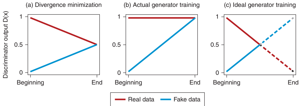
Figure 12.1 Under divergence minimization (a), the Generator is always playing catch-up with the Discriminator (because divergence is always \geq 0 ). In (b), we see what “good” NS-GAN training looks like. Again, the Generator cannot win. In (c), we can see that now the generator can win, but more importantly, the Generator always has something to strive for (and therefore recover useful gradient), no matter the stage of training.
