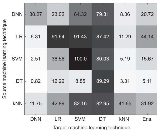
Figure 10.4 The numbers here denote the percentage of adversarial examples crafted to fool the classifier in that row that also fooled that column's classifier. The methods are deep neural networks (DNNs), logistic regression (LR), support-vector machine (SVM), decision trees (DT), nearest neighbors (kNN), and ensembles (Ens.).
