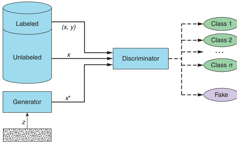
Figure 7.2 In this Semi-Supervised GAN, the Generator takes in a random noise vector z and produces a fake example x^* . The Discriminator receives three kinds of data inputs: fake data from the Generator, real unlabeled examples x , and real labeled examples (x, y) , where y is the label corresponding to the given example. The Discriminator then outputs a classification; its goal is to distinguish fake examples from the real ones and, for the real examples, identify the correct class. Notice that the portion of examples with labels is much smaller than the portion of the unlabeled data. In practice, the contrast is even starker than the one shown, with labeled data forming only a tiny fraction (often as little as 1–2%) of the training data.
