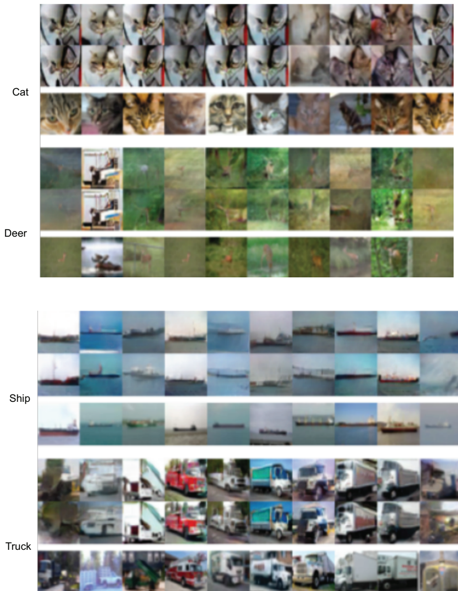
Figure 5.3 The GAN picks up on the patterns by mostly memorizing the items, which also creates an undesirable outcome indicating that the GAN has not learned much useful information and will most likely not generalize. The proof is in the images. The first two rows are pairs of duplicate samples; the last row is the nearest neighbor of the middle row in the training set. Note that these examples are very low resolution as they appear in the paper, due to a low-resolution GAN setup. (Source: “Do GANs Actually Learn the Distribution? An Empirical Study,” by Sanjeev Arora and Yi Zhang, 2017, https://arxiv.org/pdf/1706.08224v2.pdf .)
