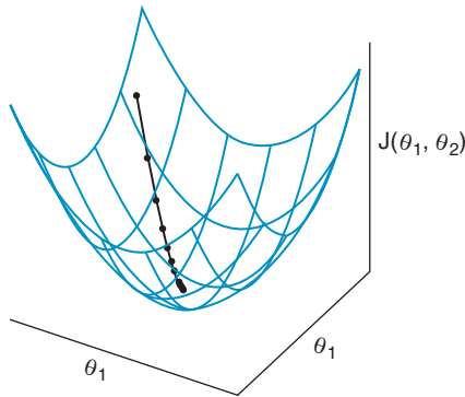
Figure 3.2 The bowl-shaped mesh represents the loss J in the parameter space \theta_1 and \theta_2 . The black dotted line illustrates the minimization of the loss in the parameter space through optimization.
