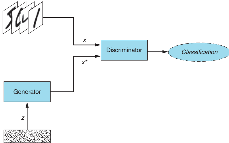
Figure 3.5 Over the course of the training iterations, the Generator learns to turn random noise input into images that look like members of the training data: the MNIST dataset of handwritten digits. Simultaneously, the Discriminator learns to distinguish the fake images produced by the Generator from the genuine ones coming from the training dataset.
