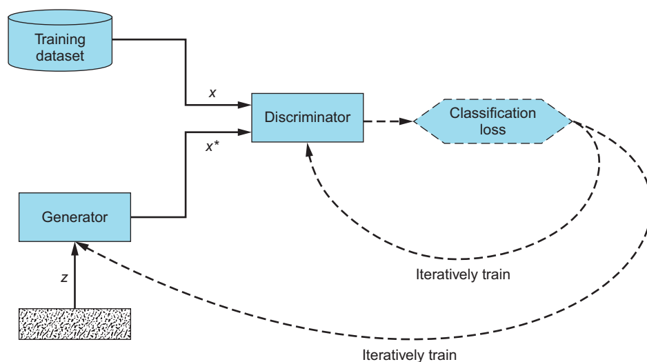
Figure 3.1 In this GAN architecture diagram, both the Generator and the Discriminator are trained using the Discriminator's loss. The Discriminator strives to minimize the loss; the Generator seeks to maximize the loss for the fake examples it produces.
