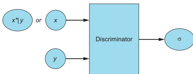
Figure 8.2 The CGAN Discriminator receives real examples along with their labels (x, y) and fake examples along with the label used to synthesize them (x^*|y, y) . The Discriminator then outputs a probability (computed by the sigmoid activation function \sigma ) indicating whether the input pair is real rather than fake.
