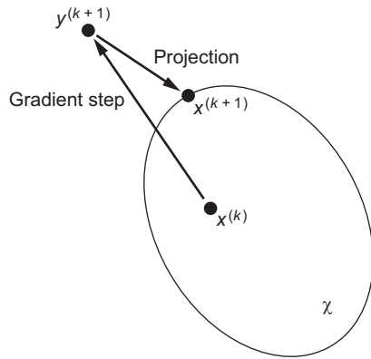
Figure 10.6 Projected gradient descent takes a step in the optimal direction, wherever it may be, and then uses projection to find the nearest equivalent point in the set of points. In this case, we are trying to ensure that we still end up with a valid picture: we take an example x^{(k)} and take the optimal step to y^{(k+1)} to then project it to a valid set of images as x^{(k+1)} .
