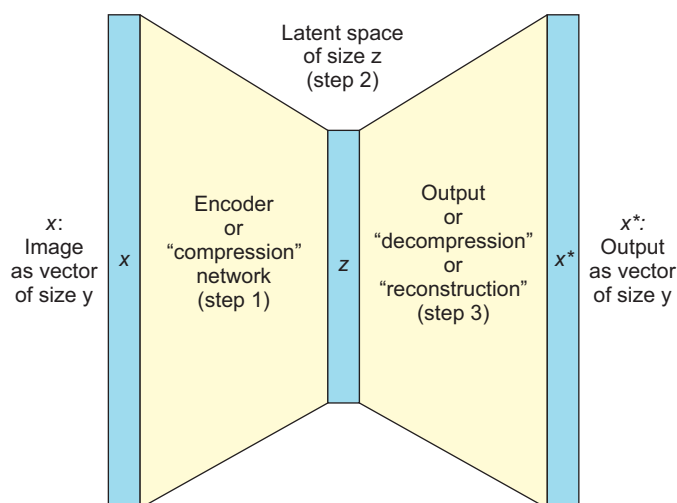
Figure 2.2 Using an autoencoder in our letter example follows these steps: (1) You compress all the things you know about a machine learning engineer, and then (2) compose that to the latent space (letter to your grandmother). When she, using her understanding of words as a decoder (3), reconstructs a (lossy) version of what that means, you get out a representation of an idea in the same space (in your grandmother's head) as the original input, which was your thoughts.
