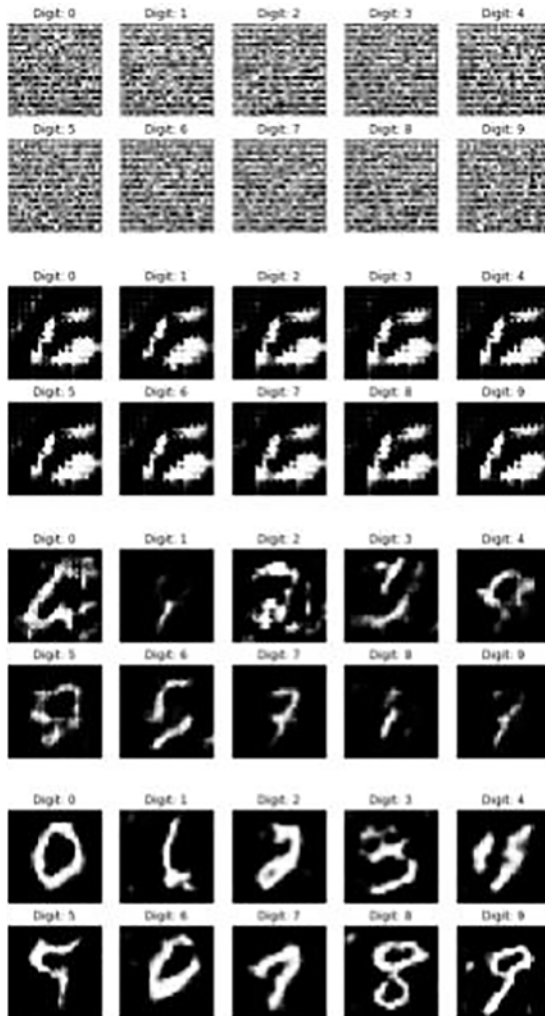
Figure 8.6 Starting from random noise, CGAN learns to produce realistic-looking numerals for each of the labels in the training dataset.
