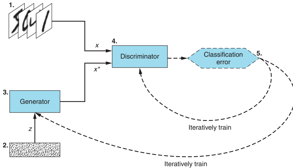
Figure 1.2 The two GAN subnetworks, their inputs and outputs, and their interactions
