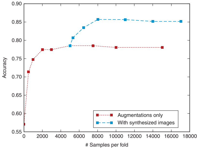
Figure 11.3 This chart shows classification accuracy as new examples are added using two dataset augmentation strategies: standard/classic data augmentation; and augmentation using synthetic examples produced by DCGAN. Using standard augmentation (dotted line), the classification performance peaks at around 80%. Using GAN-created examples (dashed line) boosts the accuracy to over 85%.
