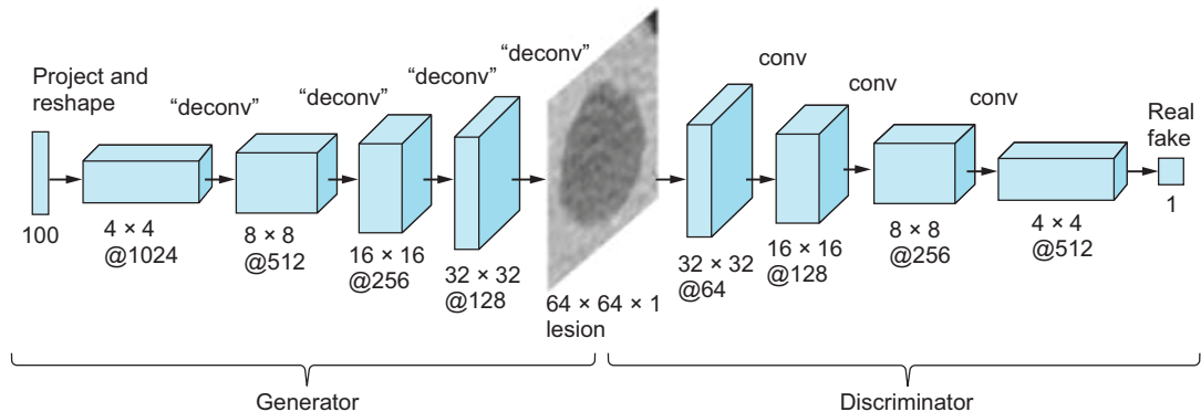
Figure 11.2 The DCGAN model architecture employed by Frid-Adar et al. to generate synthetic images of liver lesions to augment their dataset, aiming to improve classification accuracy. The model architecture is similar to the DCGAN in chapter 4, underscoring the applicability of GANs across a wide array of datasets and use cases. (Note that the figure shows only the GAN flow for fake examples.)
