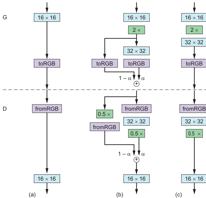
Figure 6.3 When we’ve trained for enough steps with, say, 16 \times 16 resolution (a), we introduce another transposed convolution in the Generator (G) and another convolution in the Discriminator (D) to get the “interface” between G and D to be 32 \times 32 . But we also introduce two pathways: (1 - \alpha) simple nearest neighbor upscaling, which does not have any trained parameters, but is also quite naive; and (\alpha) extra transposed convolution, which requires training but will ultimately perform much better.
