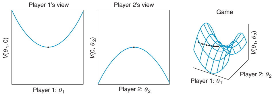
Figure 3.3 Player 1 (left) seeks to minimize V by tuning \theta_1 . Player 2 (middle) seeks to minimize -V (maximize V ) by tuning \theta_2 . The saddle-shaped mesh (right) shows the combined loss in the parameter space V(\theta_1, \theta_2) . The dotted line shows the convergence to Nash equilibrium at the center of the saddle. (Source: Goodfellow, 2019, www.iangoodfellow.com/slides/2019-05-07.pdf .)
